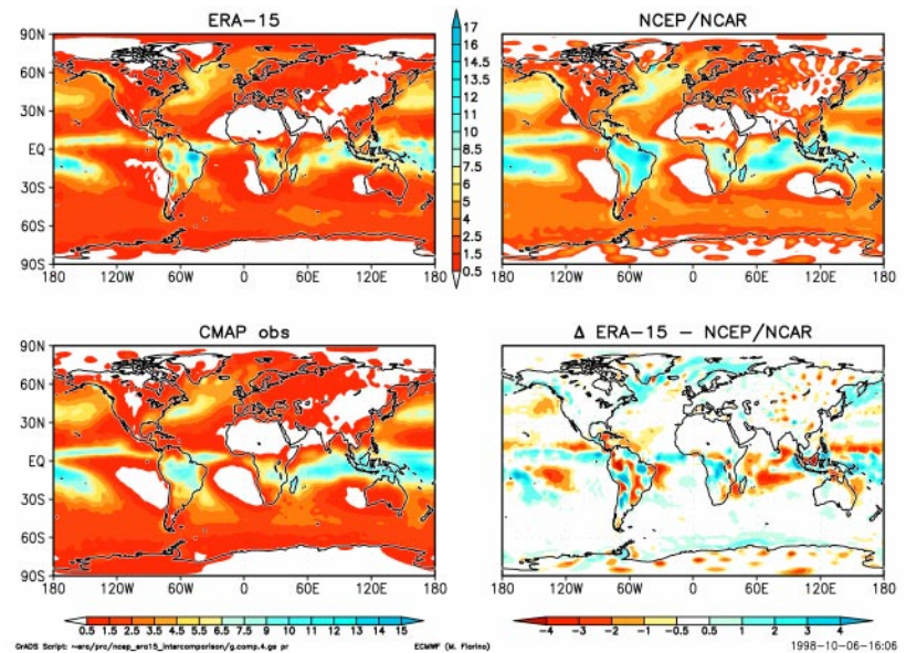
FIG. 18. Intercomparison of the mean DJF precipitation (top panels) against an analysis of observations and the difference during ERA-15 period Jan 1979–Feb 1994.
