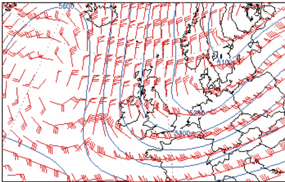
FIG. 9. The 96-h forecast valid at 0300 UTC 1 Feb, indicating the North Sea gale that caused thousands of deaths in northern Europe.
