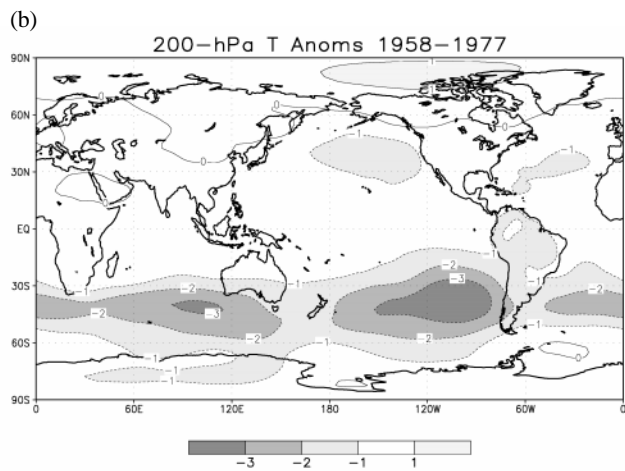
FIG. 10. (a) Cross section of globally averaged temperature anomalies showing the impact of the satellite observing system introduced in 1979. (b) Geographical distribution of the bias of the temperature at 200 hPa defined for 1958–77 and compared with the climatology defined for the years 1979–97.
