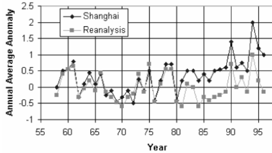
FIG. 13. Comparison of annually averaged surface temperature anomalies measured at the Shanghai Observatory (31.4° lat, 121.9° long) with the reanalysis estimated at the closest grid at 2.5° by 2.5° resolution, which is an “ocean” point.
